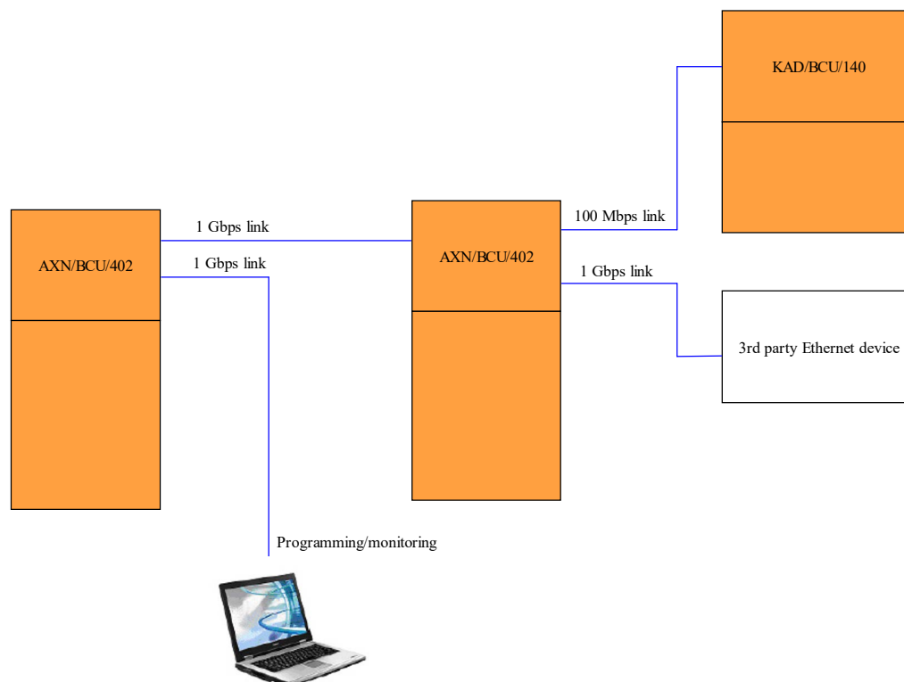
Figure 85-1: AXN network system using the internal switch from the AXN/BCU/402
