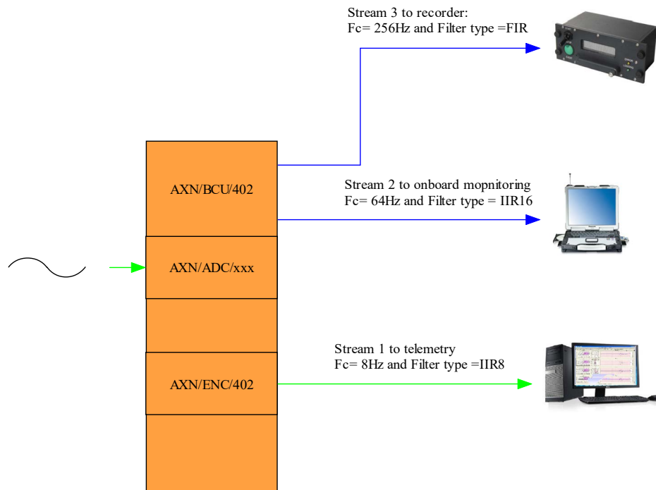
Figure 85-5: Example of 3 streams per channel
