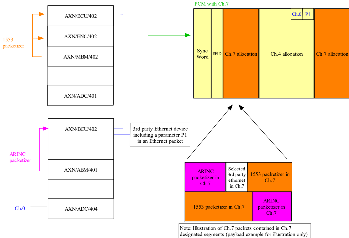
Figure 85-3: AXN network system with the AXN/ENC/402 Chapter 7
