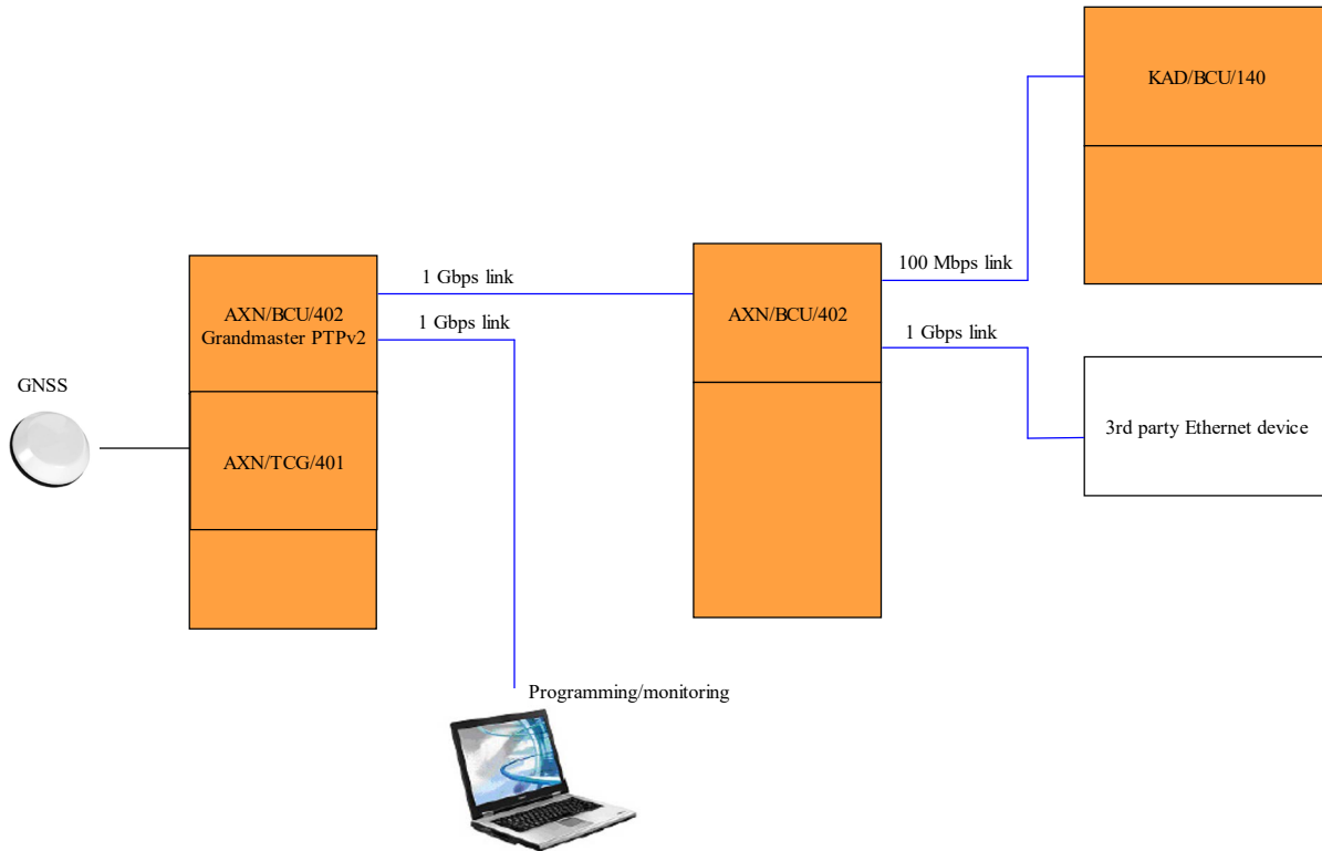
Figure 85-2: AXN network system with the AXN/BCU/402 as a PTPv2 Grandmaster
