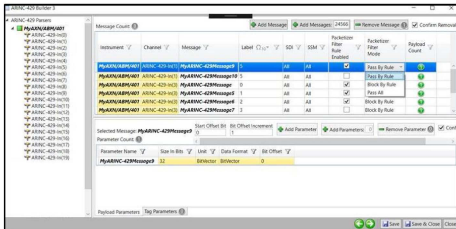
Figure 85-6: DAS Studio ARINC-429 builder showing the messages to be filtered on the packetizer
